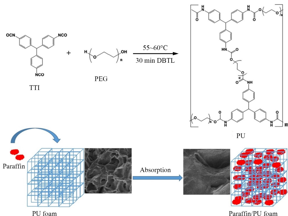
Fig. 17. Schematic illustration for preparation of PU/paraffin shape-stabilization of PCMs [84].
