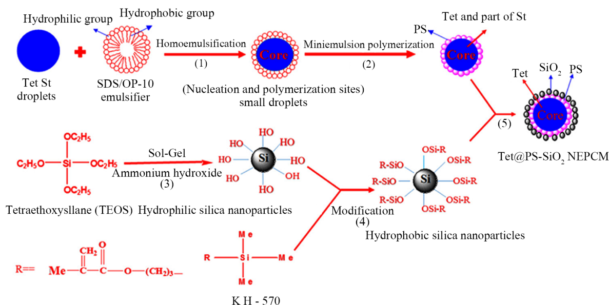
Fig. 15. Schematic of synthesis stages of n -tetradecane@polystyrene-silica NEPCM (Tet@PS-SiO 2 ) [75].
